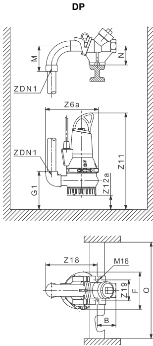
Fig. B One-pump installation on hookup auto coupling
